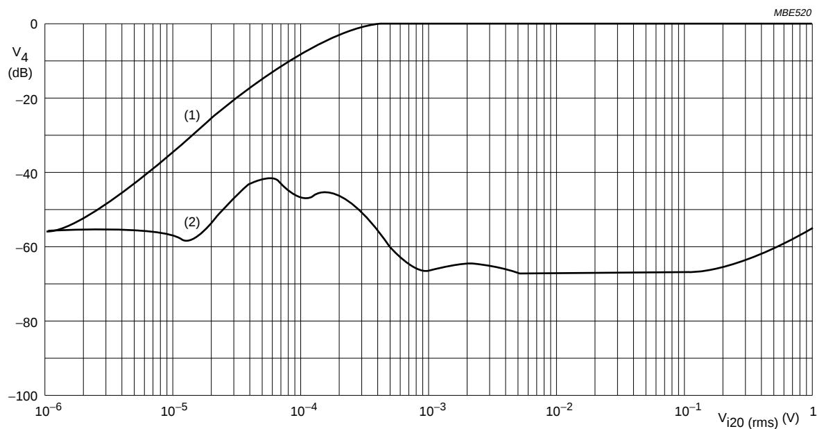
Fig.7 FM-MUTE-ON: Typical AM suppression as a function of the input signal V_{iIF} (pin 20) with \Delta f = \pm 22.5 kHz; f_m = 1 kHz; AM with f_m = 400 Hz; m = 0.3 and 250 to 15000 Hz bandwidth.
