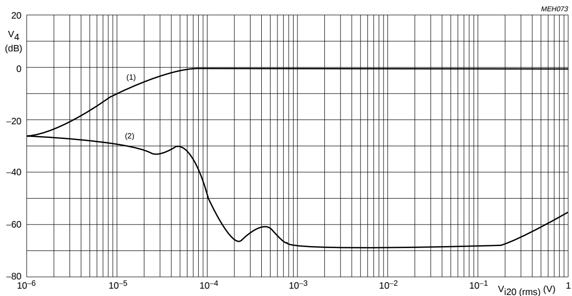
Fig.8 FM-MUTE-OFF: Typical AM suppression as a function of the input signal V_{\text{if}} (pin 20) with \Delta f = \pm 22.5 kHz; f_m = 1 kHz; AM with f_m = 400 Hz; m = 0.3 and 250 to 15000 Hz bandwidth.
